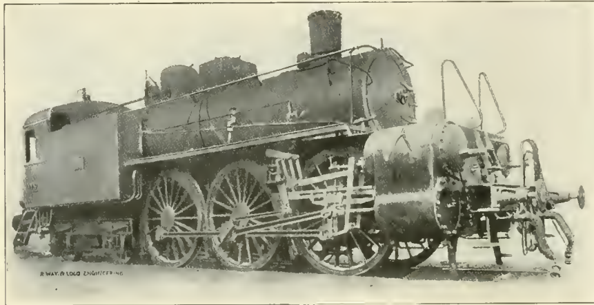
4-6-0 ENGINE ON THE ADRIATIC RAILWAY OF ITALY.
